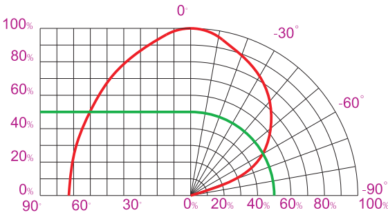
Directive Characteristics
